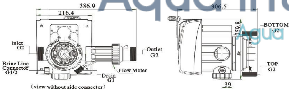
Structure Chart of N74A3 ( 63610 )
