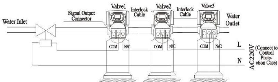
Figure 3-4 Wiring of Solenoid Valve in Inlet
