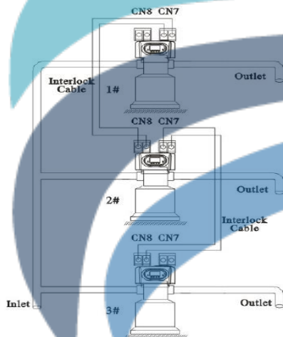
Figure 3-12 Interlock system
