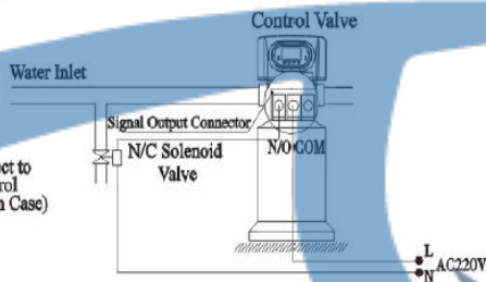
Figure 3-3 Wiring of Pressure Relief Port
