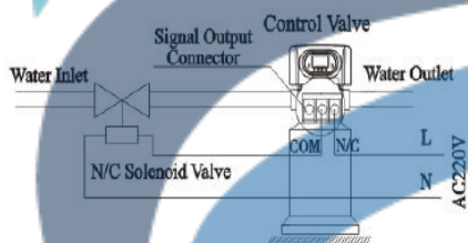
Figure 3-2 Wiring of Solenoid Valve on Inlet
